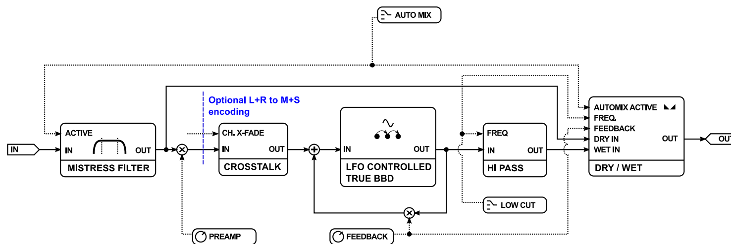
Antresol effect diagram
