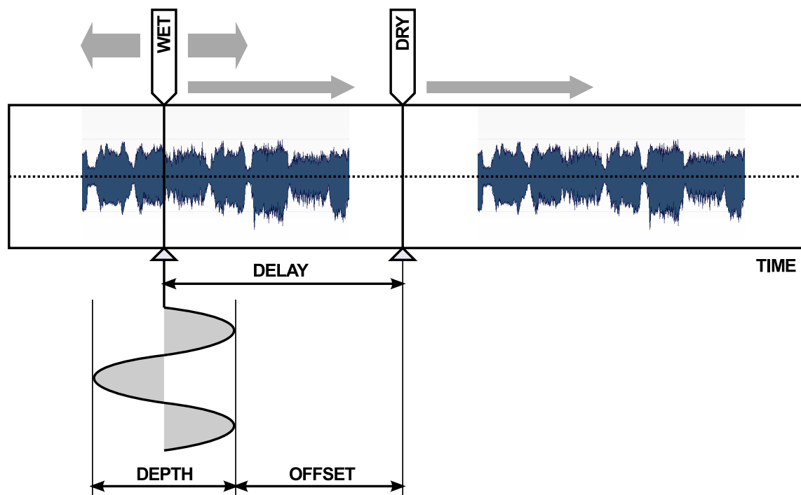
LFO controlling the delay time
